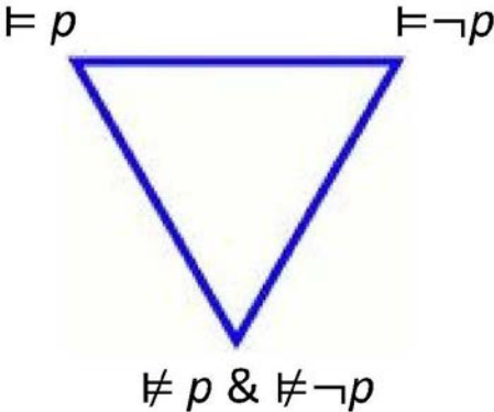
FIGURE 4 – DOUBLE TURNSTILE TAUTOLOGICAL TRIANGLE OF CONTRARIETY
