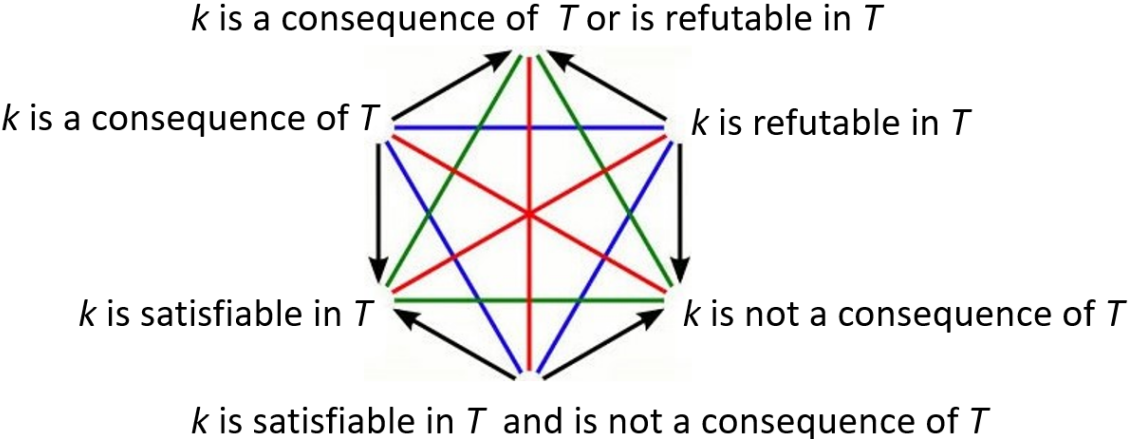
FIGURE 13 – TERMINOLOGICAL MODEL-THEORETICAL HEXAGON - NO TRUTH VERSION
