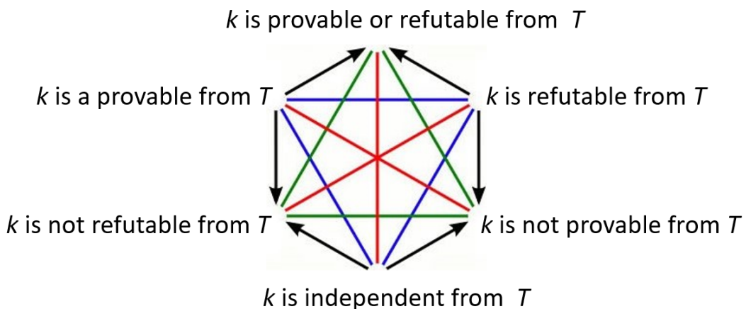
FIGURE 10 – TERMINOLOGICAL PROOF-THEORETICAL HEXAGON
