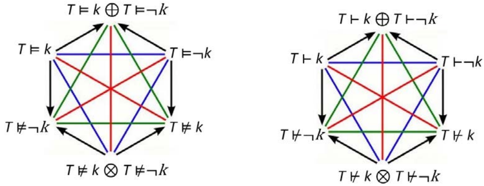
FIGURE 9 – TURNSTILE CONSEQUENTIAL HEXAGONS
