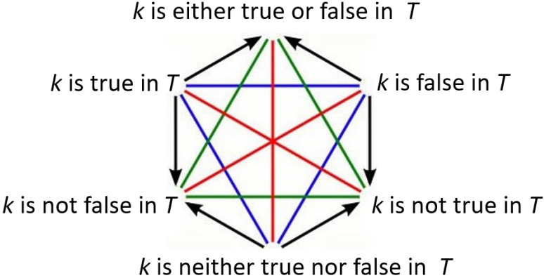
FIGURE 12 – TERMINOLOGICAL MODEL-THEORETICAL HEXAGON -TRUTH VERSION
