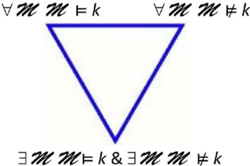
FIGURE 7 – MODEL-THEORETICAL TRIANGLE OF CONTRARIETY
