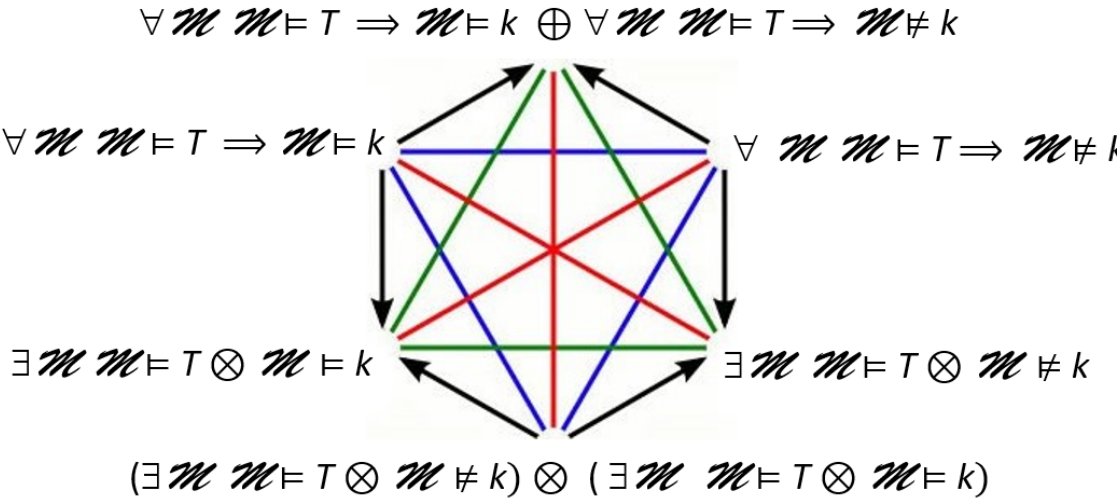
FIGURE 11 – MODEL-THEORETICAL HEXAGON
